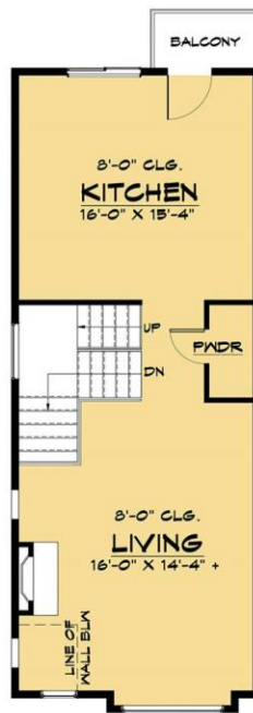
MAIN FLOOR PLAN
